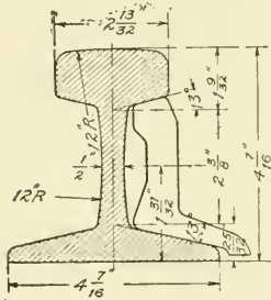
Fig. 222. Section of 65-pound T Rail
